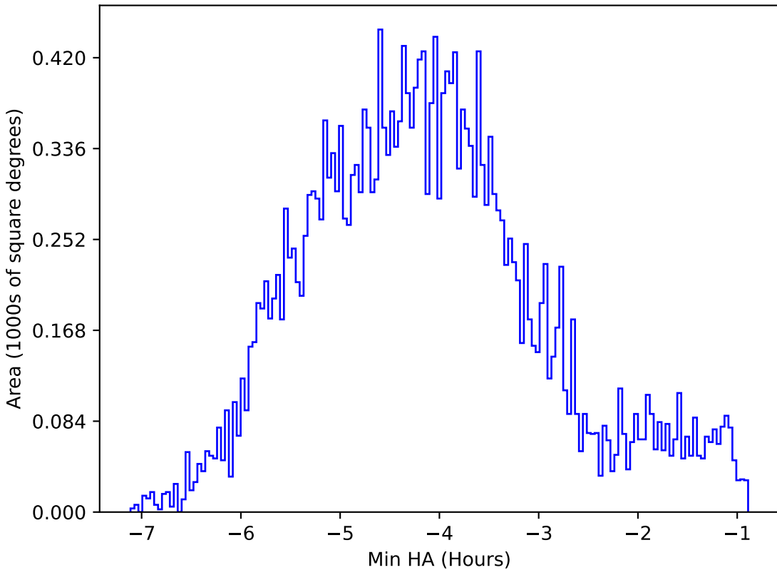
too_elab_r16_d3_griz_v3.4_10yrs All sky r band: Min HA
