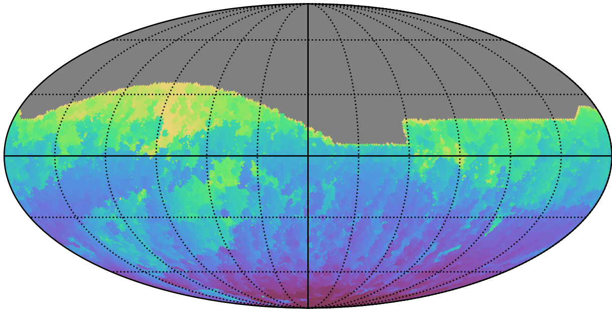
too_elab_r16_d3_griz_v3.4_10yrs All sky i band: Min HA
