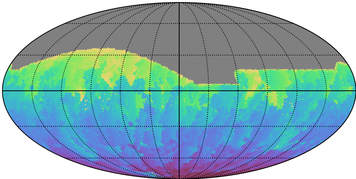
too_elab_r16_d3_griz_v3.4_10yrs All sky g band: Min HA
