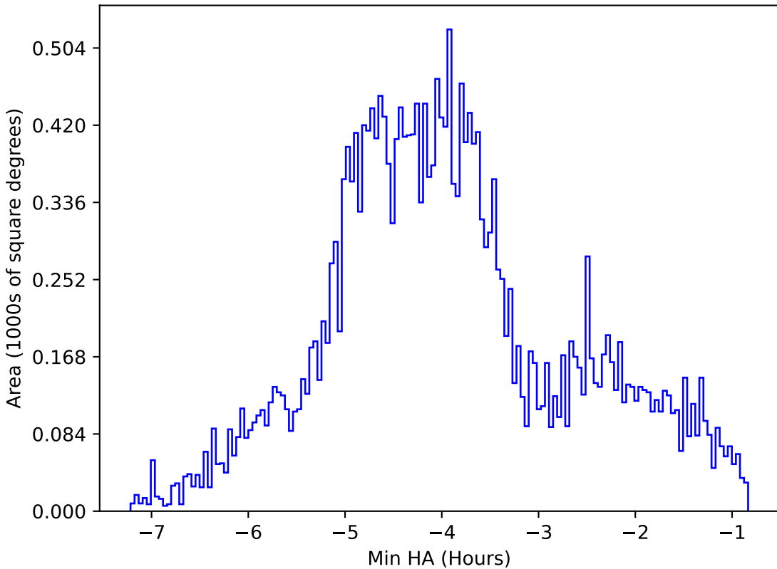
too_elab_r16_d3_griz_v3.4_10yrs All sky g band: Min HA
