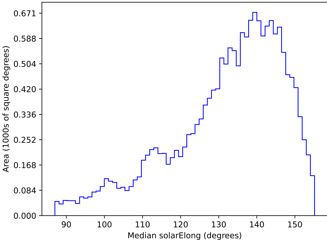
too_elab_r16_d3_griz_v3.4_10yrs WFD u band: Median solarElong
