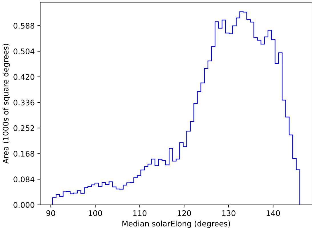
too_elab_r16_d3_griz_v3.4_10yrs WFD i band: Median solarElong
