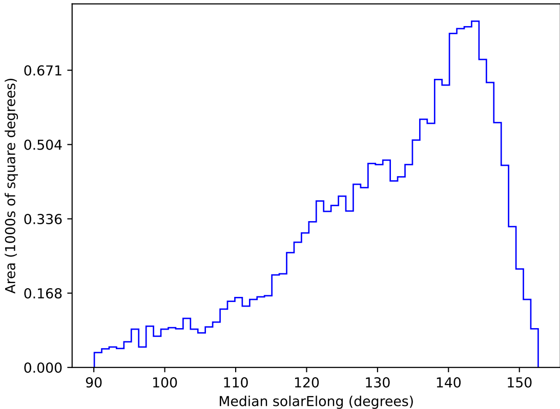
too_elab_r16_d3_griz_v3.4_10yrs WFD g band: Median solarElong
