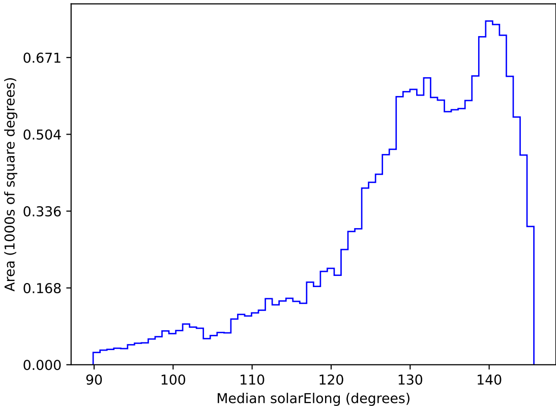
too_elab_r16_d3_griz_v3.4_10yrs WFD all bands: Median solarElong
