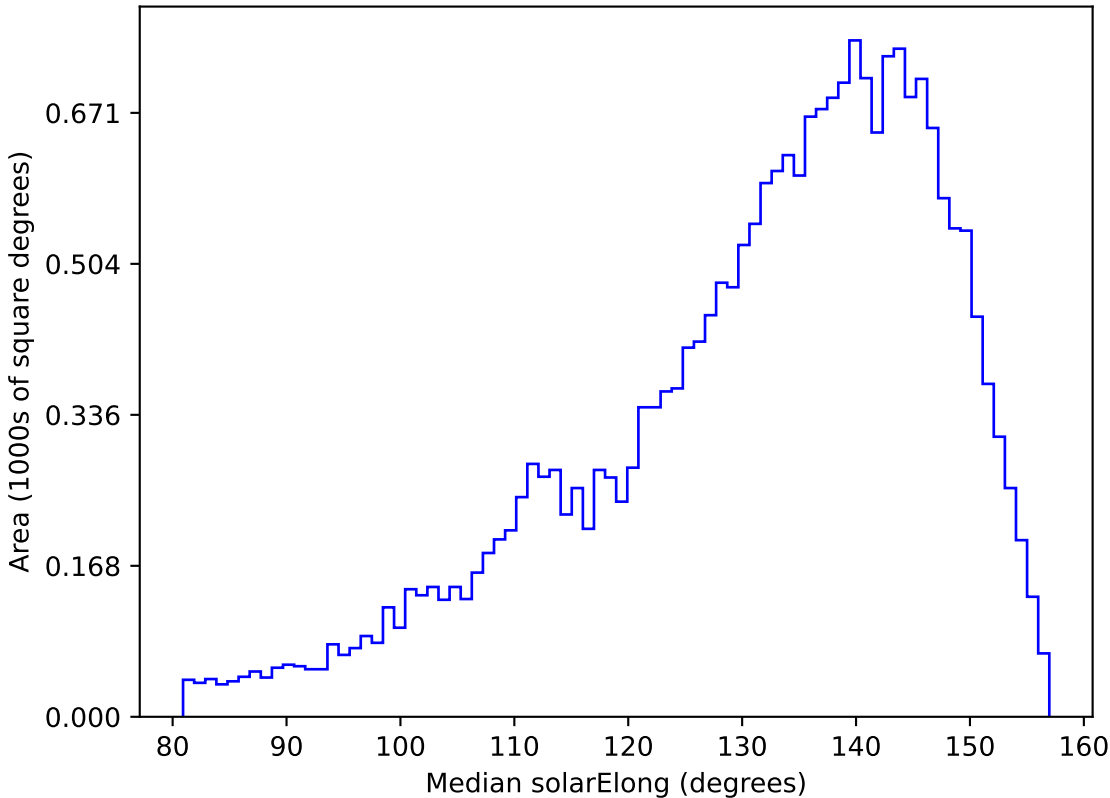
too_elab_r16_d3_griz_v3.4_10yrs All sky u band: Median solarElong
