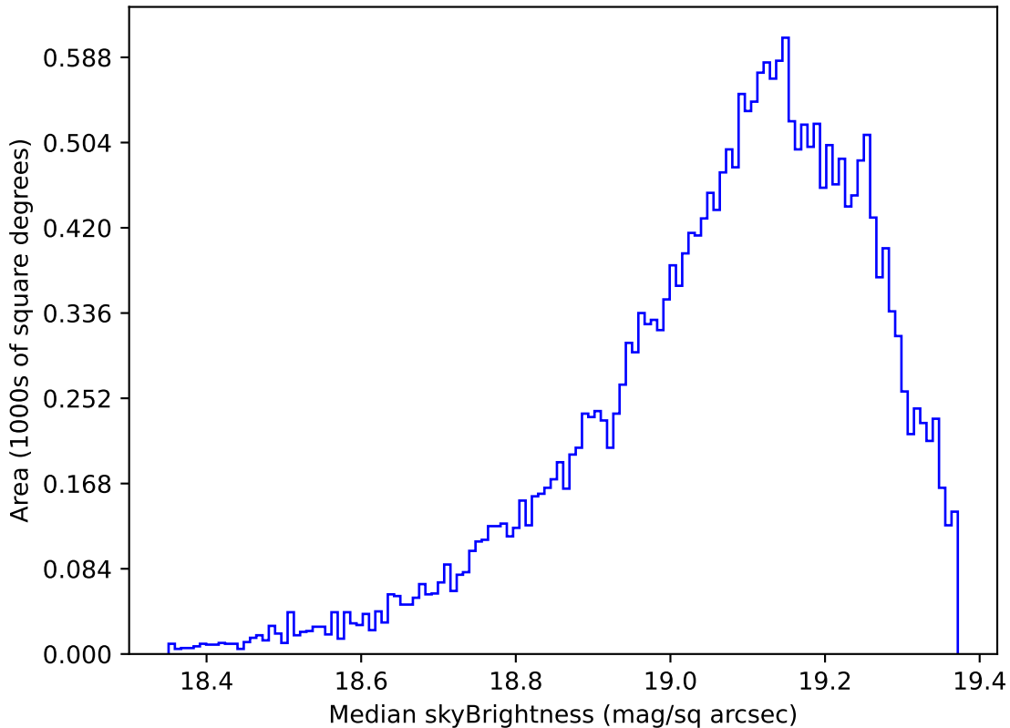
too_elab_r16_d3_griz_v3.4_10yrs Yr 1 z band: Median skyBrightness
