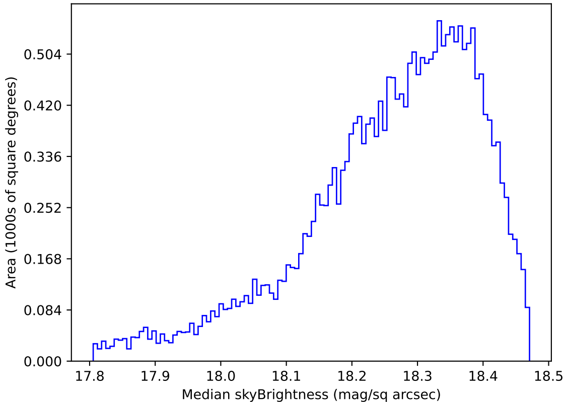
too_elab_r16_d3_griz_v3.4_10yrs Yr 1 y band: Median skyBrightness
