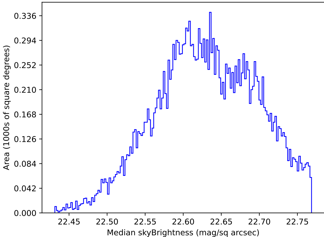
too_elab_r16_d3_griz_v3.4_10yrs Yr 1 u band: Median skyBrightness
