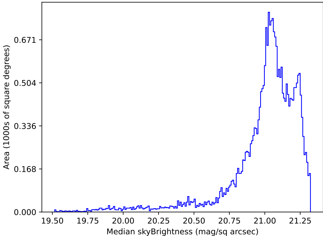
too_elab_r16_d3_griz_v3.4_10yrs Yr 1 r band: Median skyBrightness
