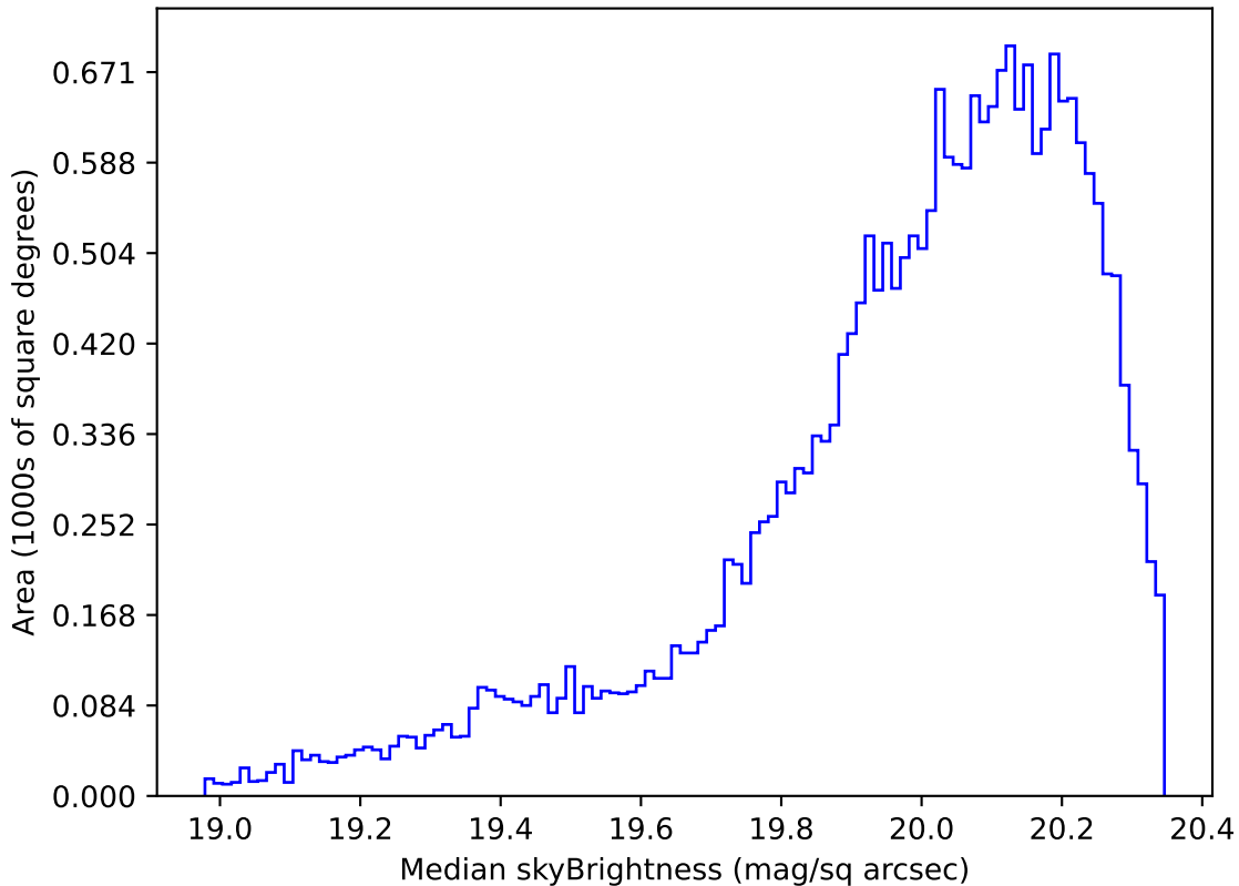
too_elab_r16_d3_griz_v3.4_10yrs Yr 1 i band: Median skyBrightness
