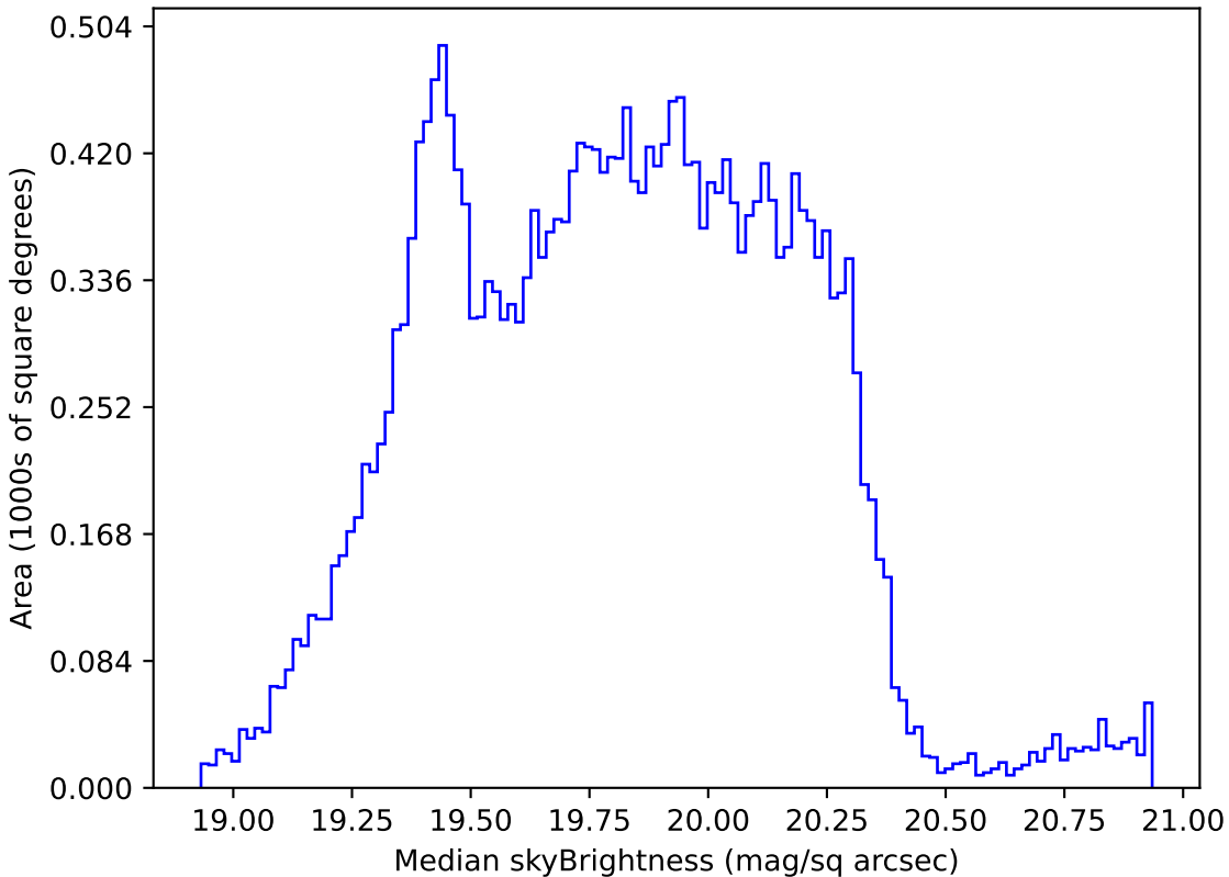
too_elab_r16_d3_griz_v3.4_10yrs Yr 1 all bands: Median skyBrightness
