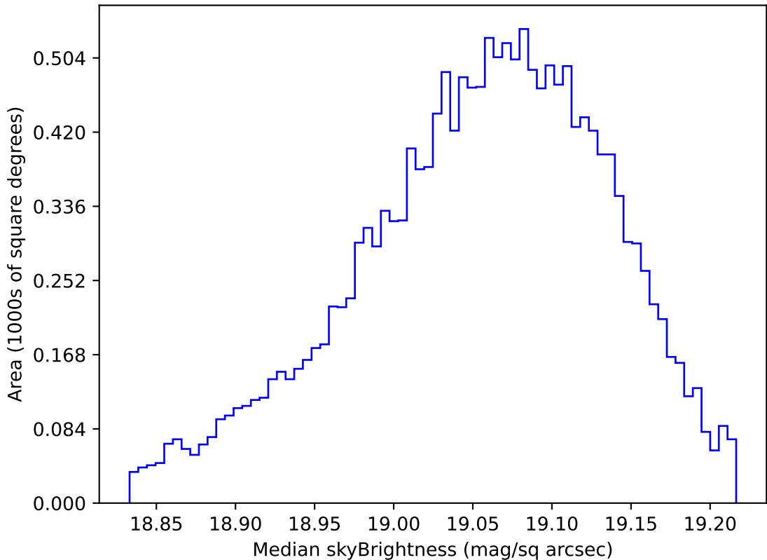
too_elab_r16_d3_griz_v3.4_10yrs WFD z band: Median skyBrightness
