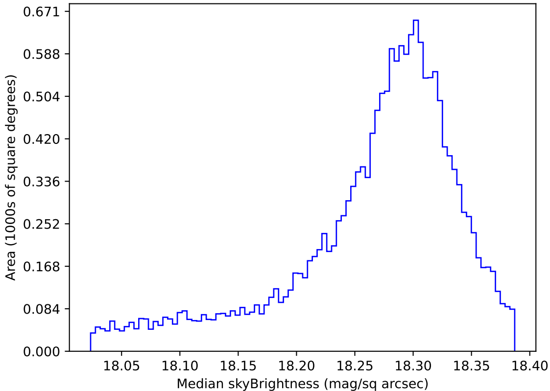
too_elab_r16_d3_griz_v3.4_10yrs WFD y band: Median skyBrightness
