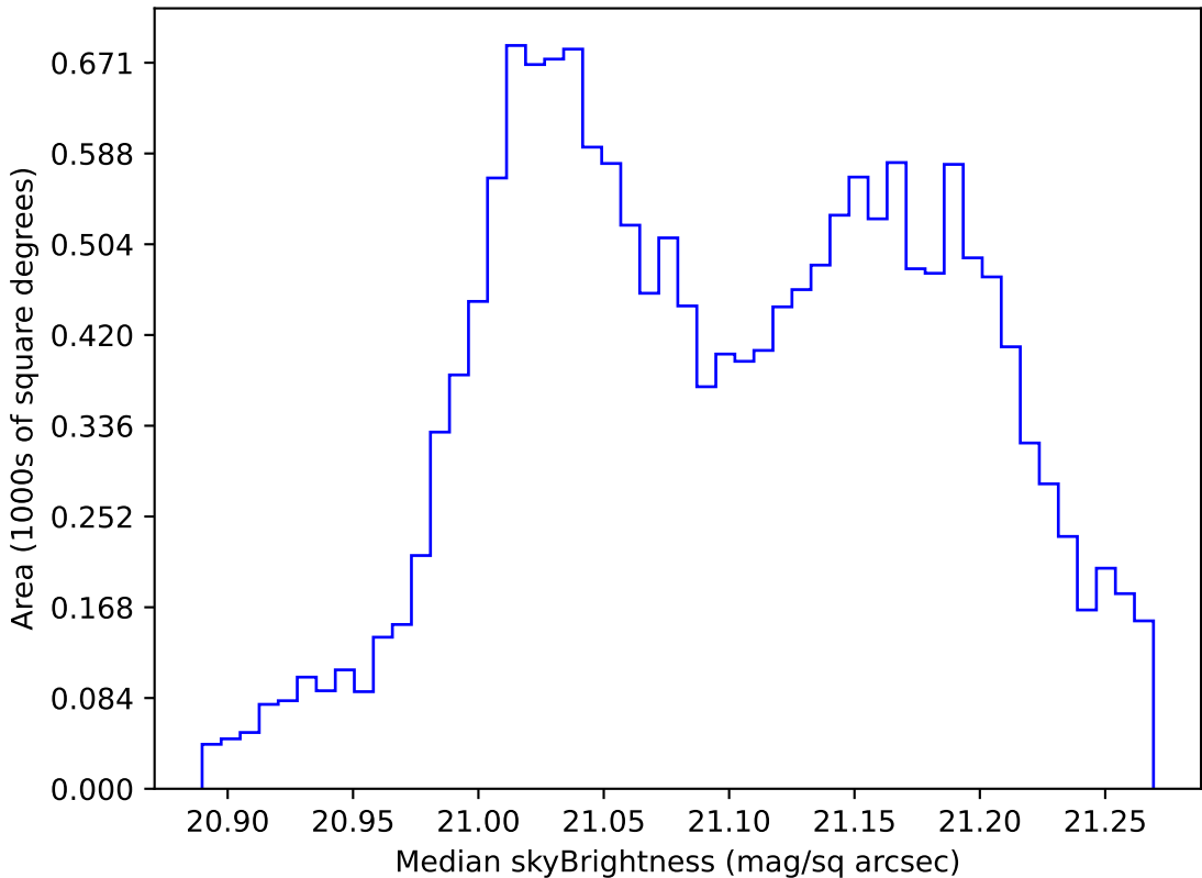
too_elab_r16_d3_griz_v3.4_10yrs WFD r band: Median skyBrightness
