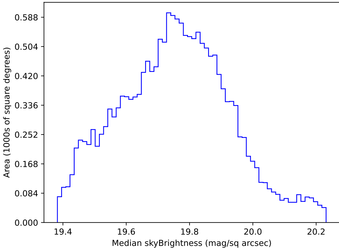
too_elab_r16_d3_griz_v3.4_10yrs WFD all bands: Median skyBrightness
