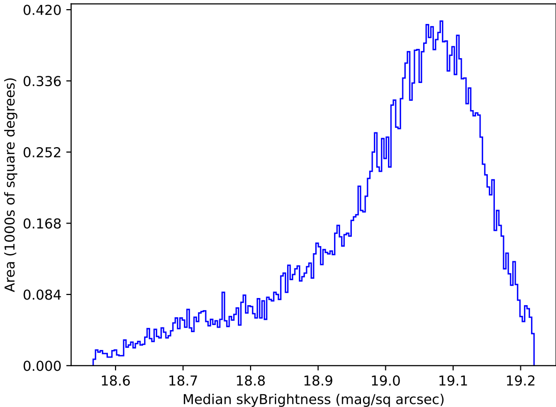
too_elab_r16_d3_griz_v3.4_10yrs All sky z band: Median skyBrightness
