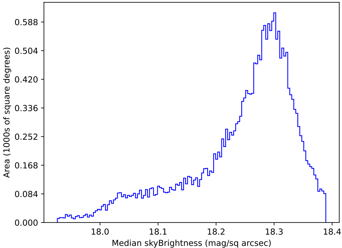
too_elab_r16_d3_griz_v3.4_10yrs All sky y band: Median skyBrightness
