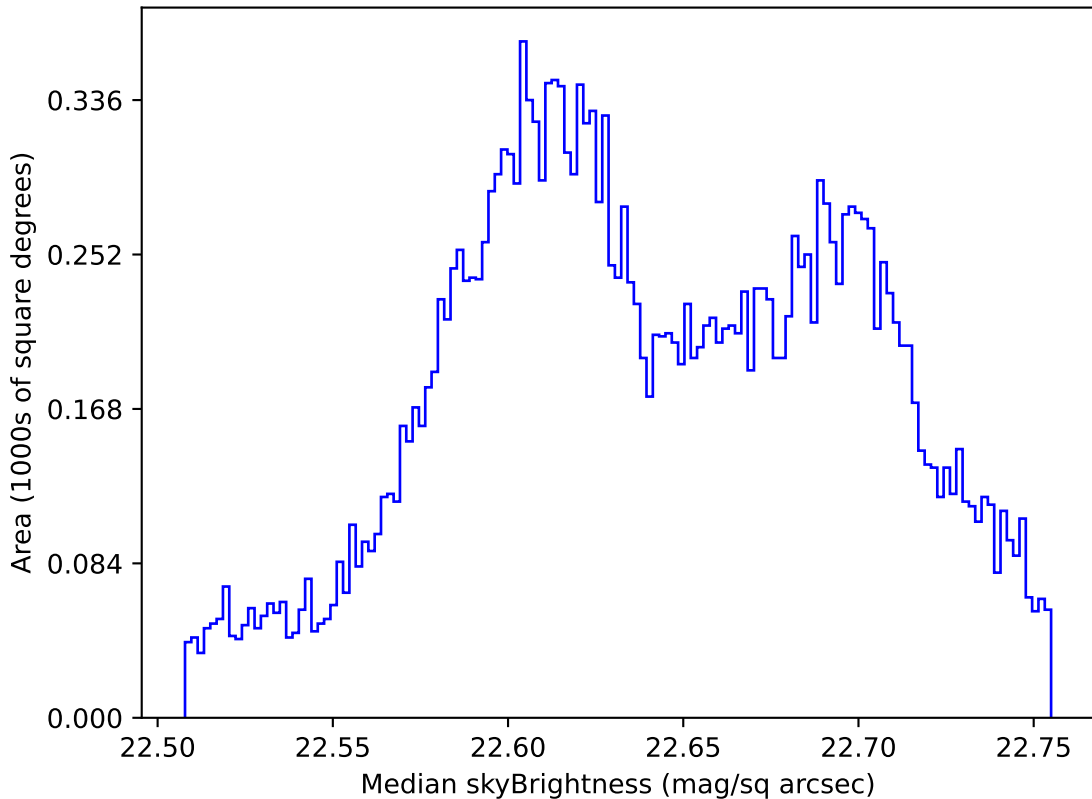
too_elab_r16_d3_griz_v3.4_10yrs All sky u band: Median skyBrightness
