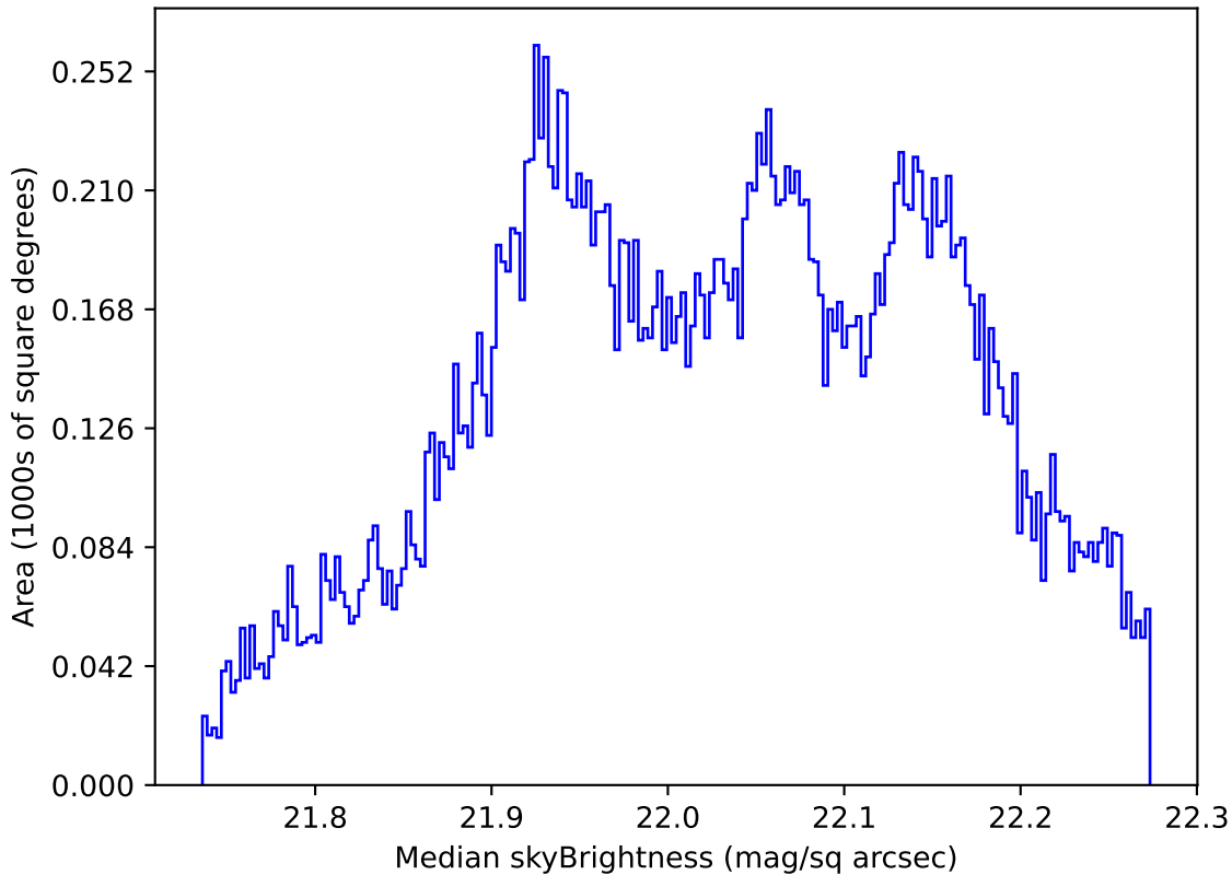
too_elab_r16_d3_griz_v3.4_10yrs All sky g band: Median skyBrightness
