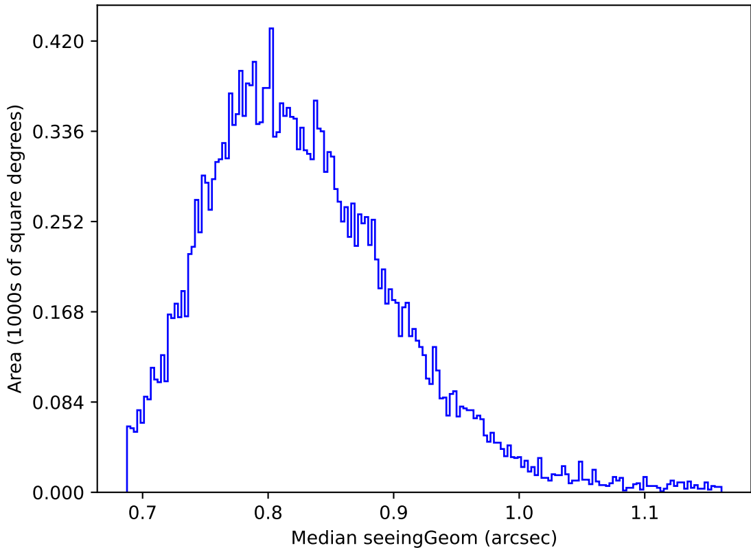
too_elab_r16_d3_griz_v3.4_10yrs Yr 1 y band: Median seeingGeom
