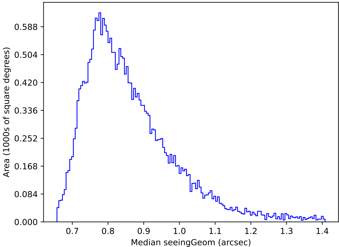
too_elab_r16_d3_griz_v3.4_10yrs Yr 1 r band: Median seeingGeom
