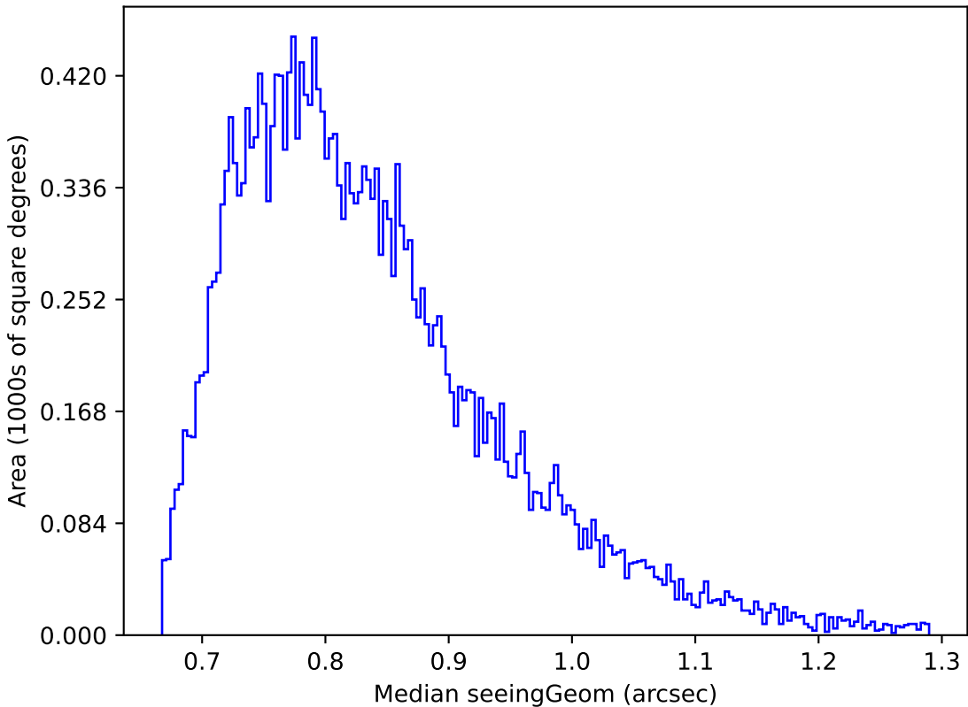
too_elab_r16_d3_griz_v3.4_10yrs Yr 1 i band: Median seeingGeom
