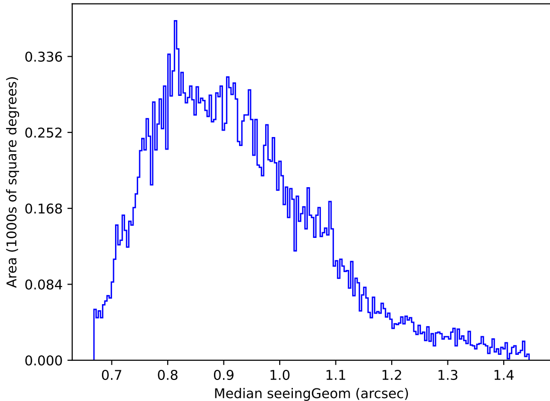
too_elab_r16_d3_griz_v3.4_10yrs Yr 1 g band: Median seeingGeom
