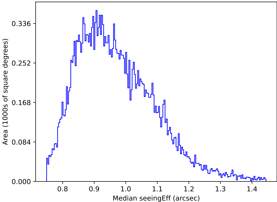
too_elab_r16_d3_griz_v3.4_10yrs Yr 1 z band: Median seeingEff
