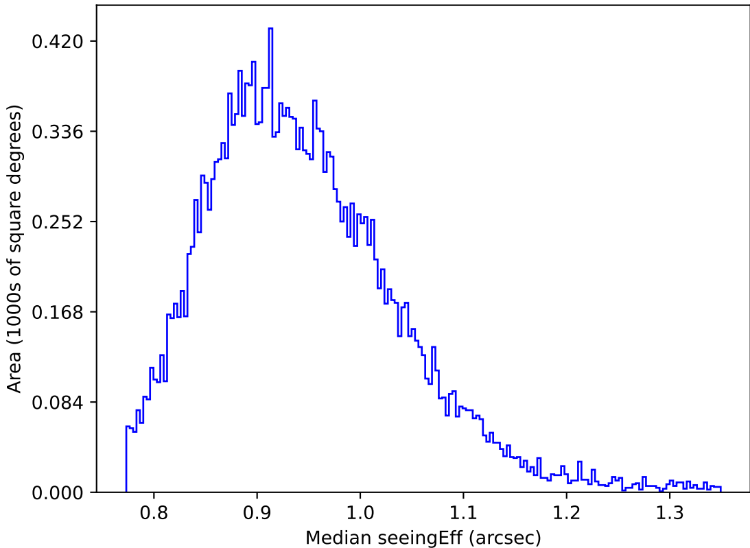
too_elab_r16_d3_griz_v3.4_10yrs Yr 1 y band: Median seeingEff
