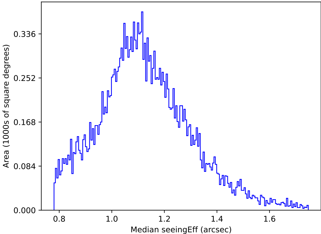
too_elab_r16_d3_griz_v3.4_10yrs Yr 1 u band: Median seeingEff
