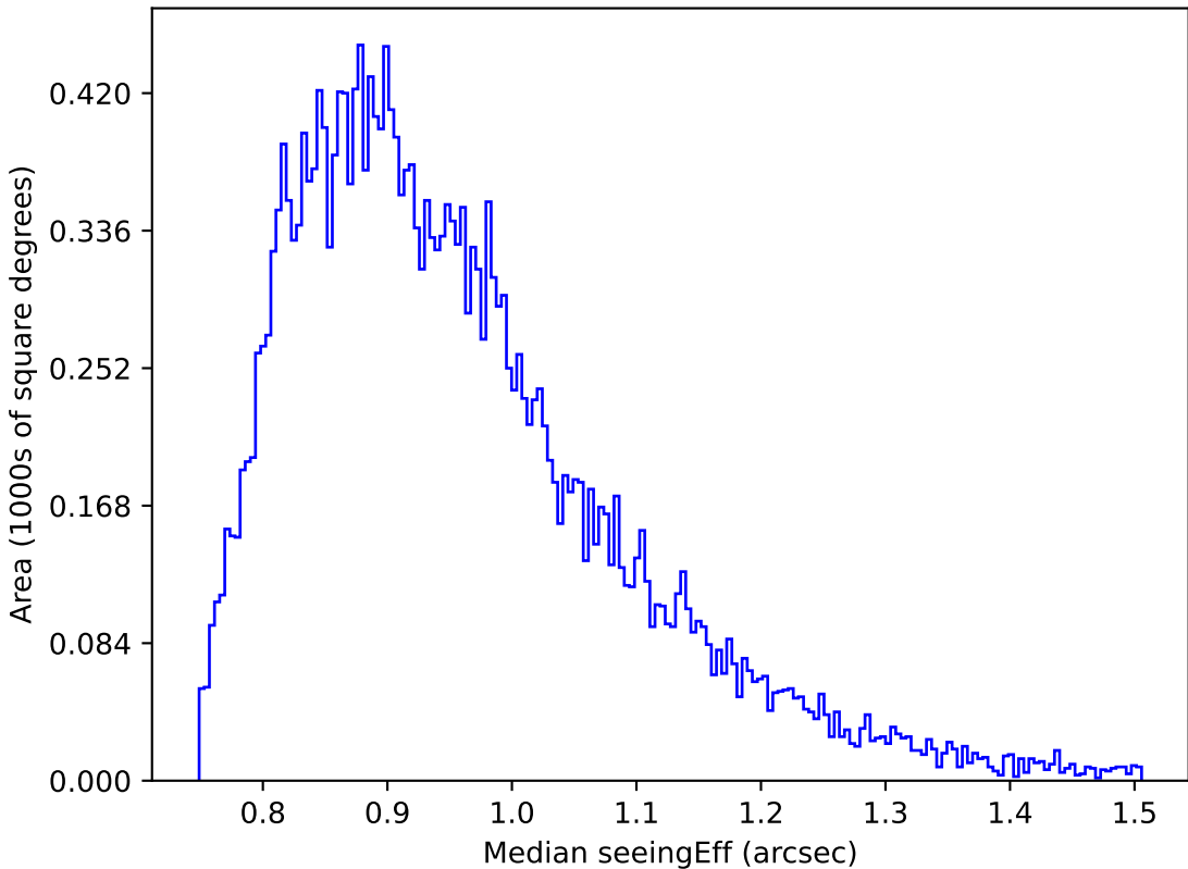
too_elab_r16_d3_griz_v3.4_10yrs Yr 1 i band: Median seeingEff
