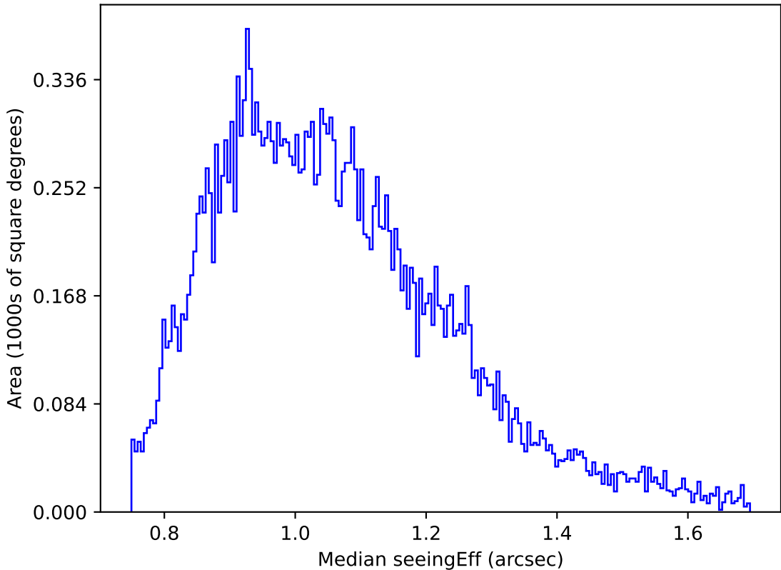
too_elab_r16_d3_griz_v3.4_10yrs Yr 1 g band: Median seeingEff
