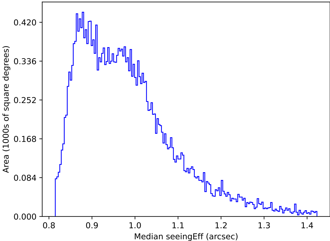
too_elab_r16_d3_griz_v3.4_10yrs Yr 1 all bands: Median seeingEff
