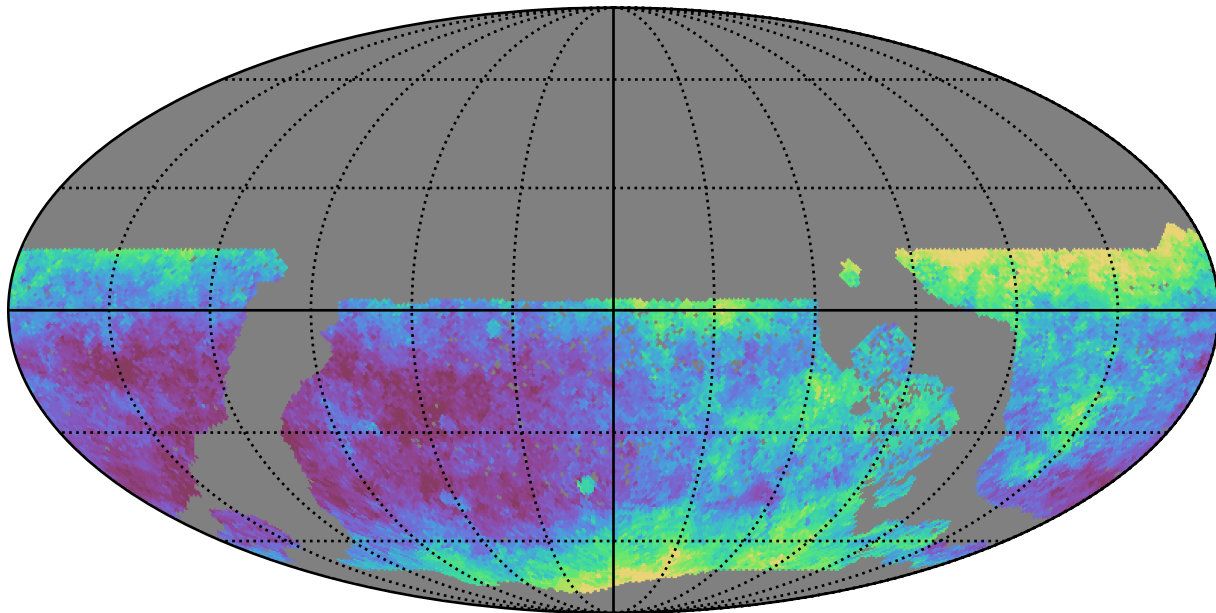
too_elab_r16_d3_griz_v3.4_10yrs WFD y band: Median seeingEff
