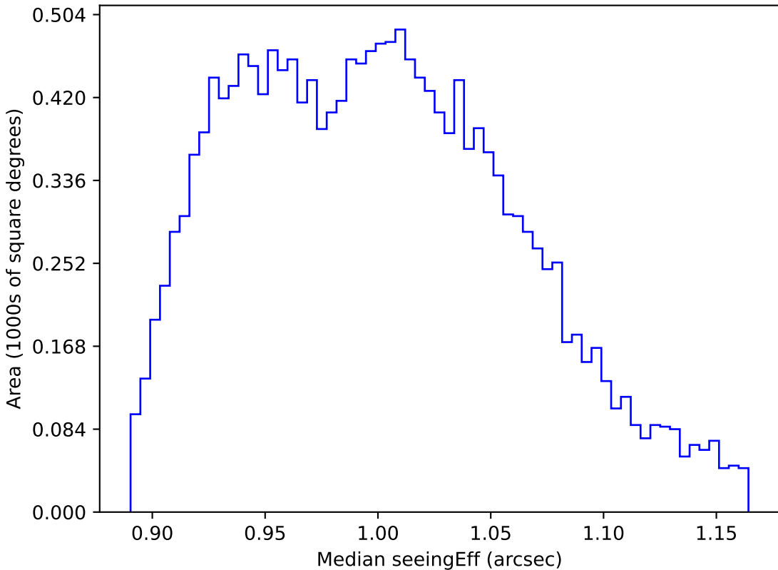
too_elab_r16_d3_griz_v3.4_10yrs WFD y band: Median seeingEff
