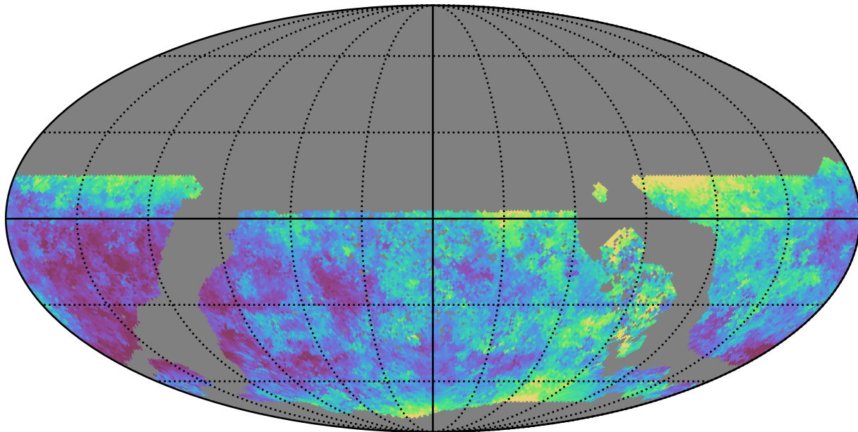
too_elab_r16_d3_griz_v3.4_10yrs WFD u band: Median seeingEff
