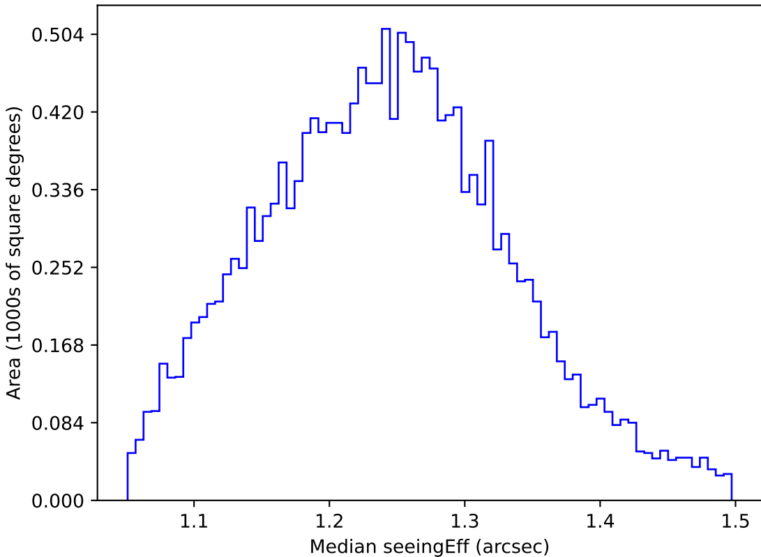
too_elab_r16_d3_griz_v3.4_10yrs WFD u band: Median seeingEff
