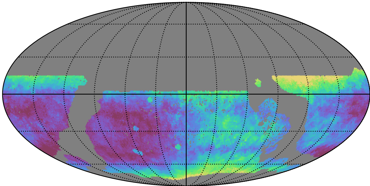
too_elab_r16_d3_griz_v3.4_10yrs WFD r band: Median seeingEff
