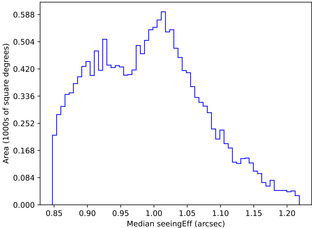
too_elab_r16_d3_griz_v3.4_10yrs WFD i band: Median seeingEff
