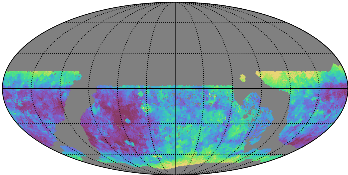
too_elab_r16_d3_griz_v3.4_10yrs WFD g band: Median seeingEff
