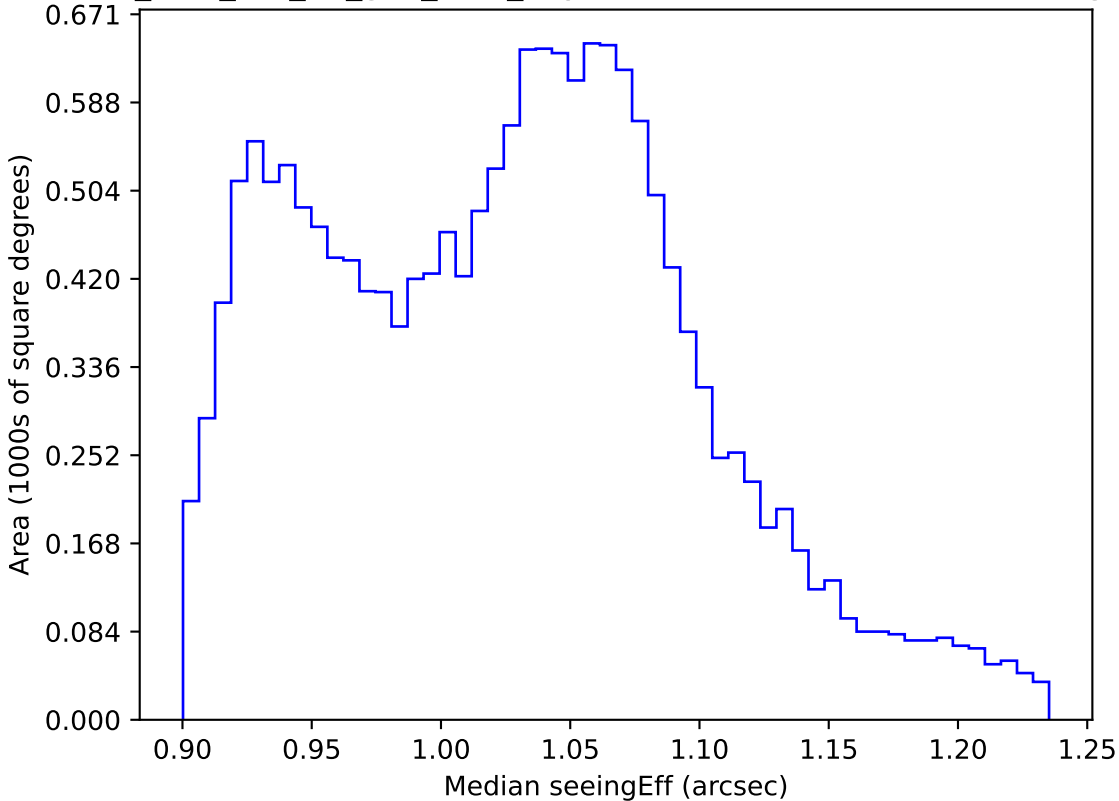
too_elab_r16_d3_griz_v3.4_10yrs WFD all bands: Median seeingEff
