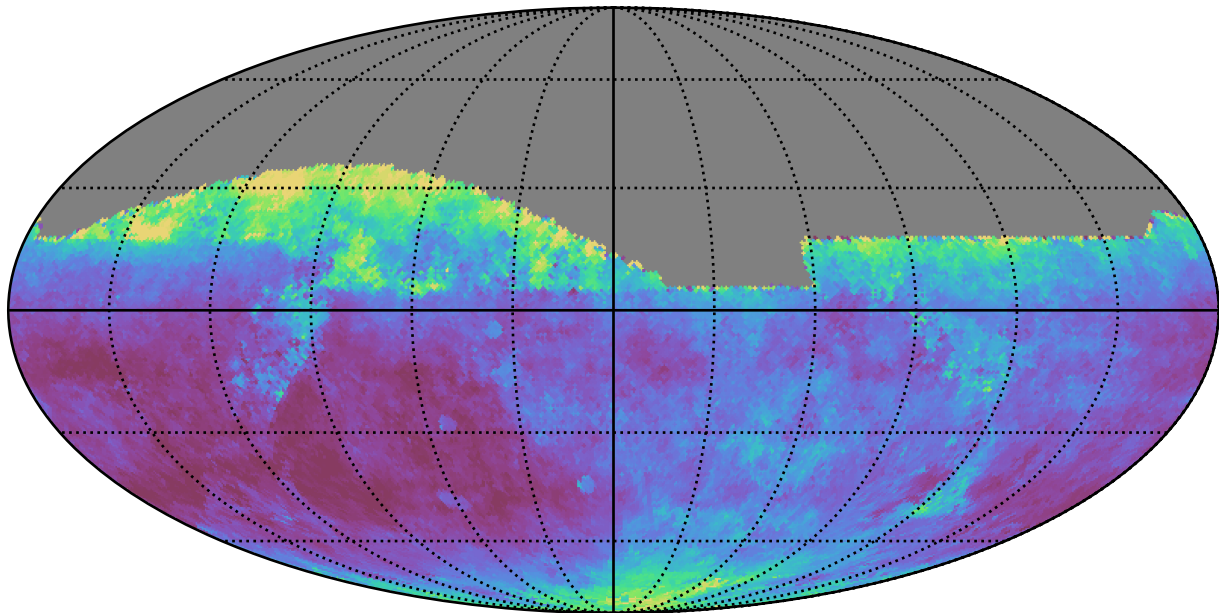
too_elab_r16_d3_griz_v3.4_10yrs All sky z band: Median seeingEff
