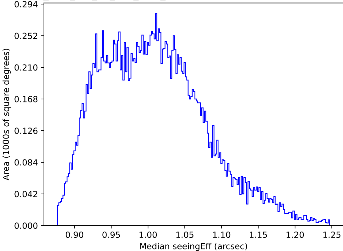
too_elab_r16_d3_griz_v3.4_10yrs All sky y band: Median seeingEff
