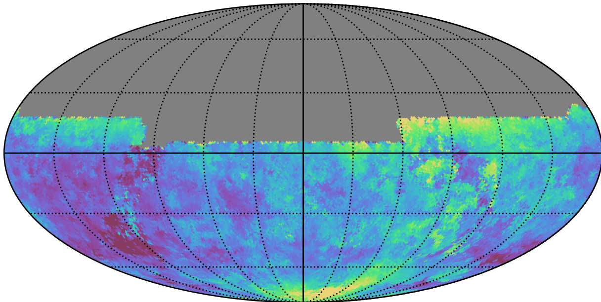
too_elab_r16_d3_griz_v3.4_10yrs All sky u band: Median seeingEff
