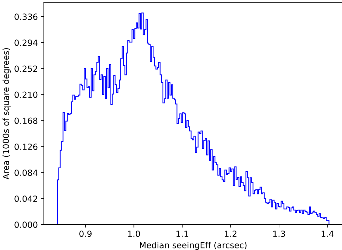
too_elab_r16_d3_griz_v3.4_10yrs All sky i band: Median seeingEff
