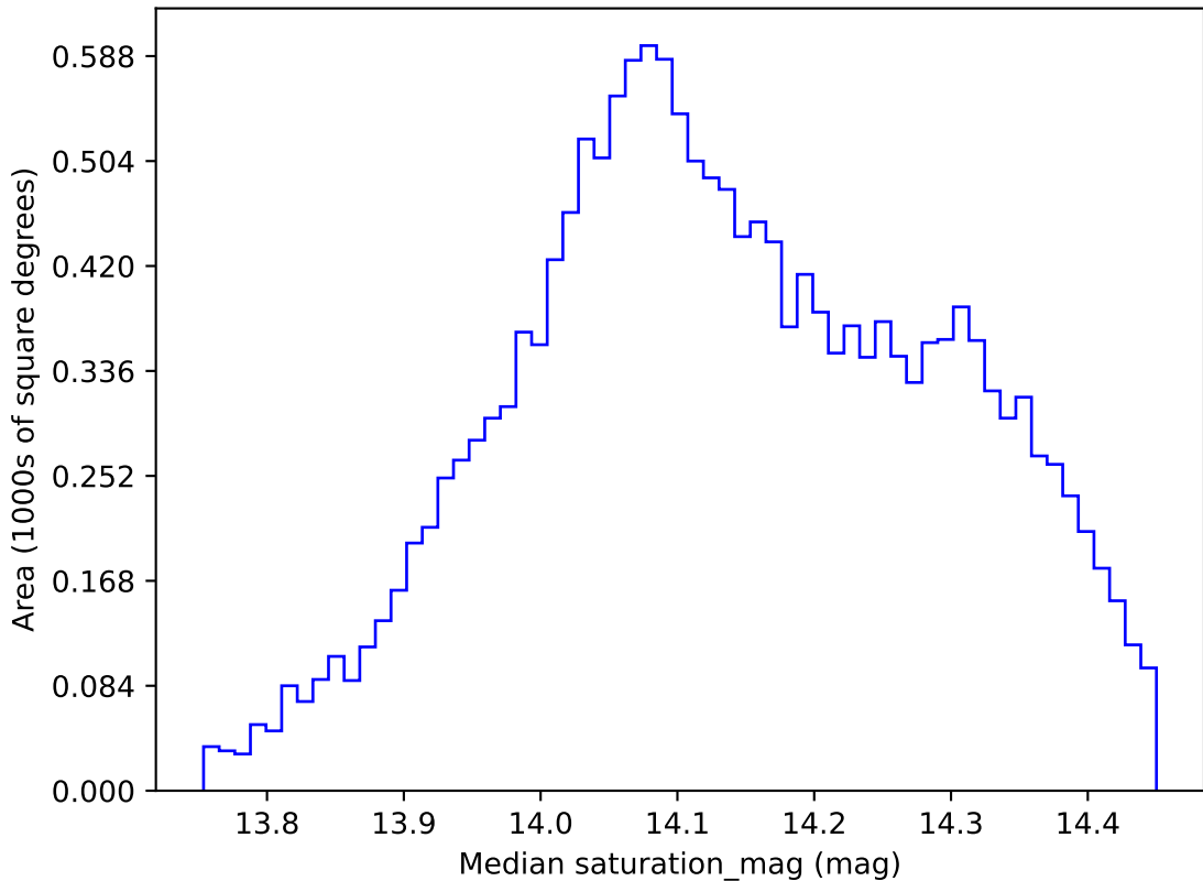
too_elab_r16_d3_griz_v3.4_10yrs WFD z band: Median saturation_mag
