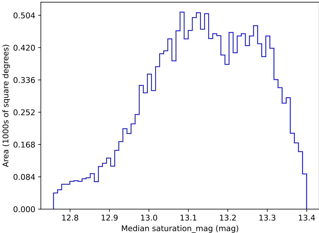
too_elab_r16_d3_griz_v3.4_10yrs WFD y band: Median saturation_mag
