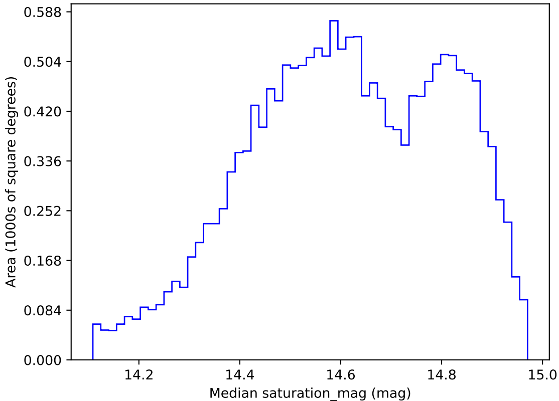
too_elab_r16_d3_griz_v3.4_10yrs WFD r band: Median saturation_mag
