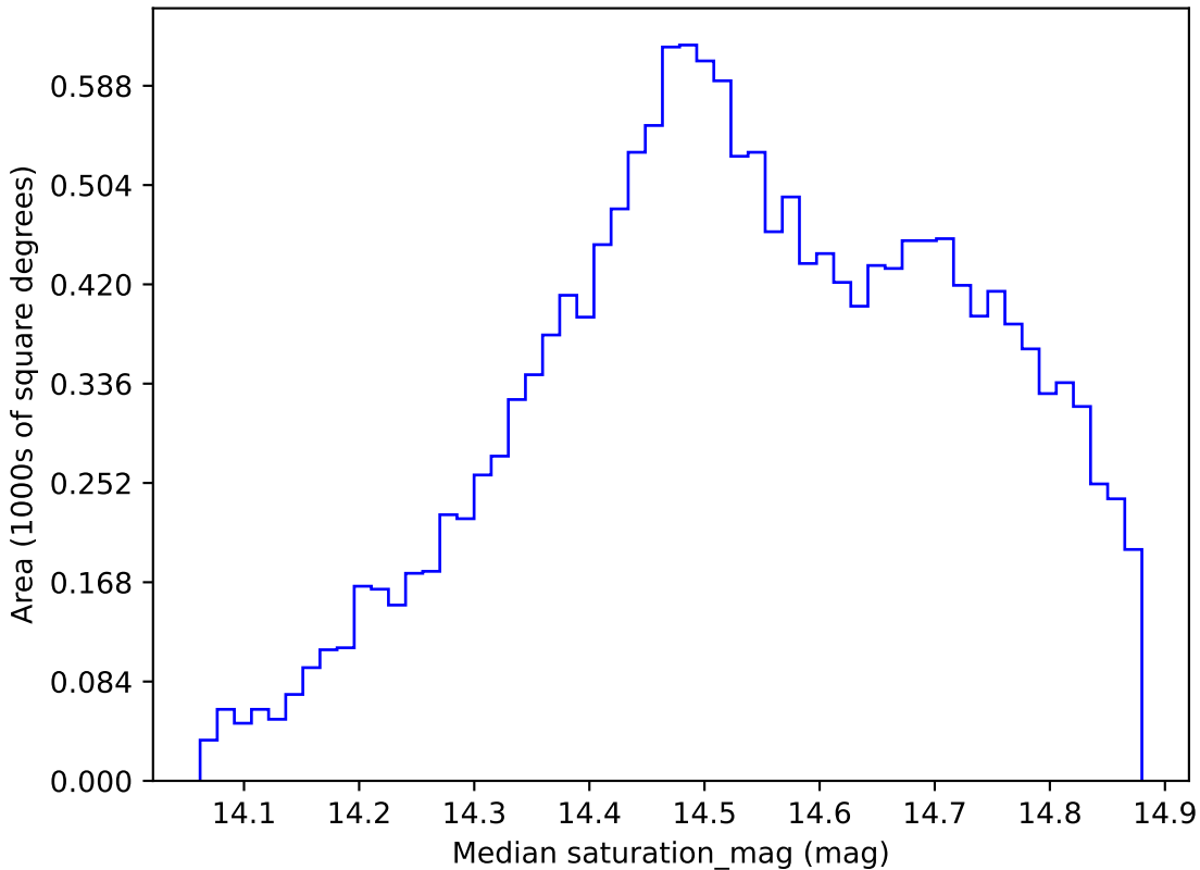
too_elab_r16_d3_griz_v3.4_10yrs WFD i band: Median saturation_mag
