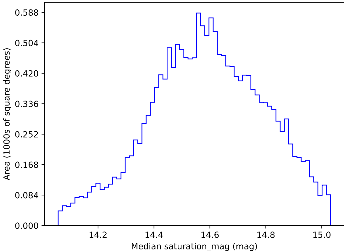
too_elab_r16_d3_griz_v3.4_10yrs WFD g band: Median saturation_mag
